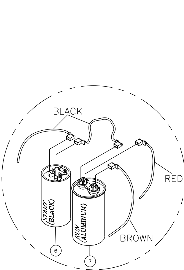
CAPACITOR TERMINAL ASSEMBLY
